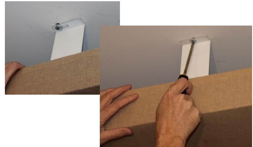
After installing toggle bolts into ceiling, slide the bracket onto the bolt and tighten.
